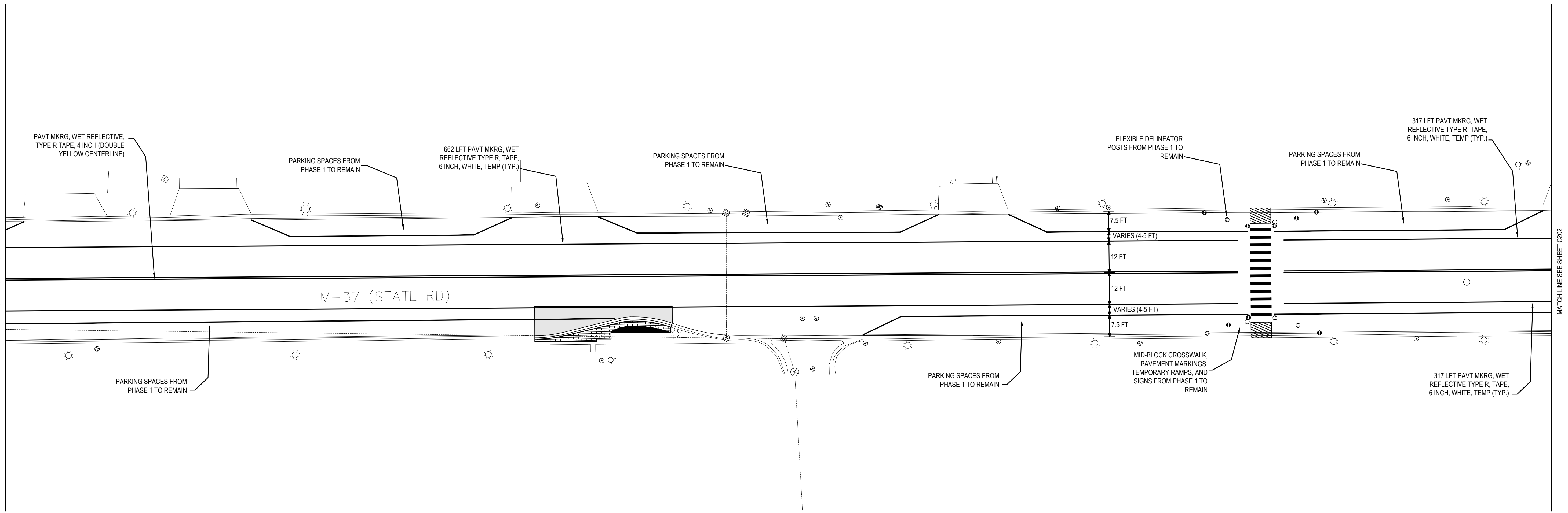
M-37 (STATE ROAD) 1" = 20'
