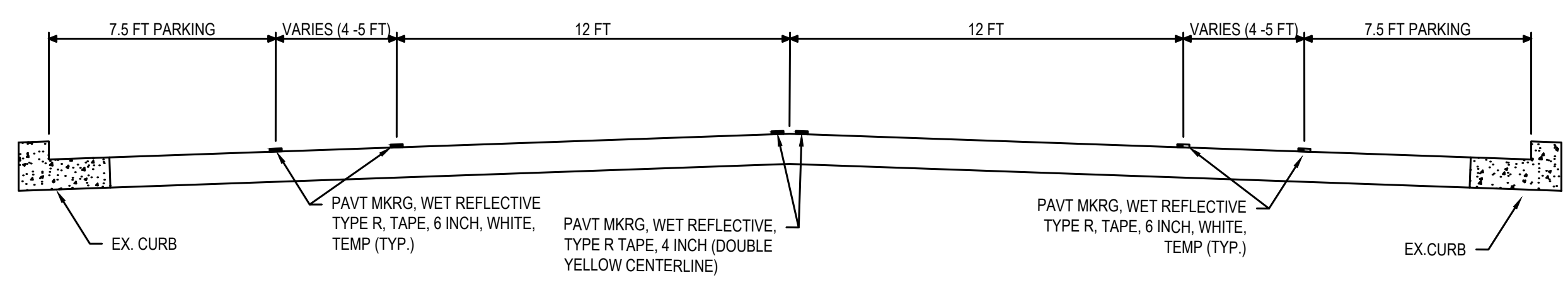
M-37 (STATE ROAD) TYPICAL CROSS-SECTION (ALTERNATIVE 1)
